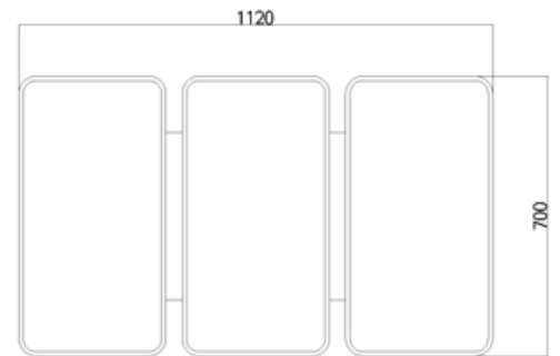
■ 콤비 II/III 거실등 150W Size_ W1120×D700×H85 Lamp_ LED 150W
