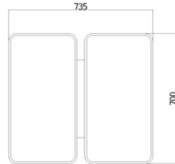
■ 콤비 II/III 거실등 100W Size_ W735×D700×H85 Lamp_ LED 100W
